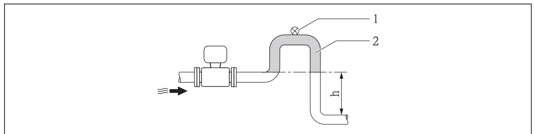
11 Installation in a down pipe
