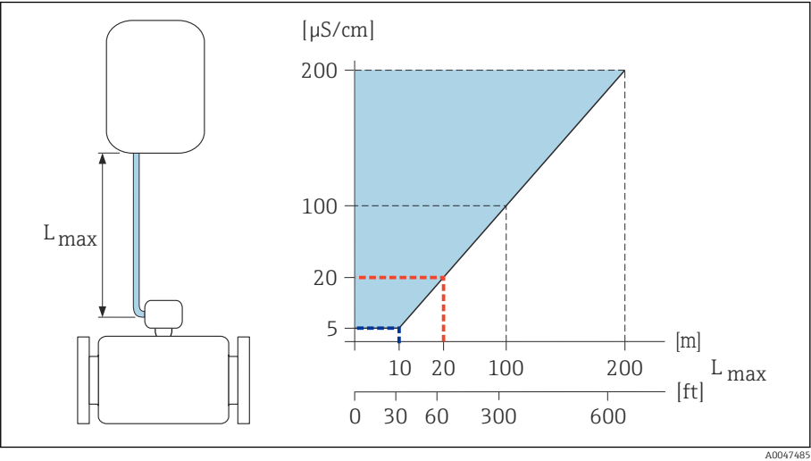
4 Permitted length of connecting cable
