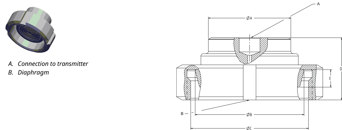
Figure 51: SLS Hygienic Dairy Process Connection Female Thread Seal per DIN 11851
