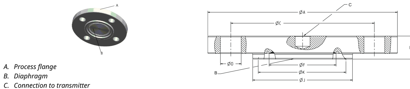
Figure 41: FVW Flush Flanged Type Seal - EN1092-1 Type C
