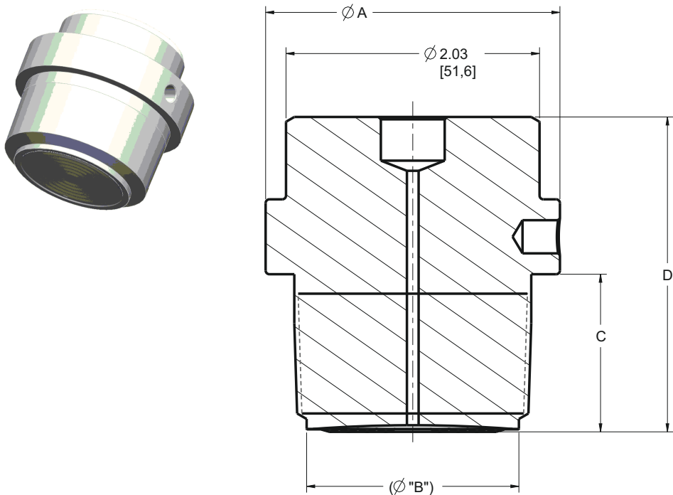
Figure 43: HTS Male Threaded Seal
