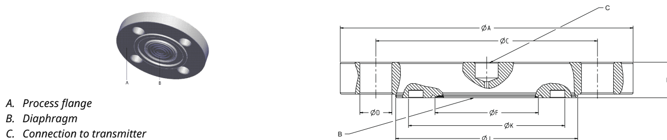
Figure 40: FUW Flush Flanged Type Seal - EN1092-1 Type D
