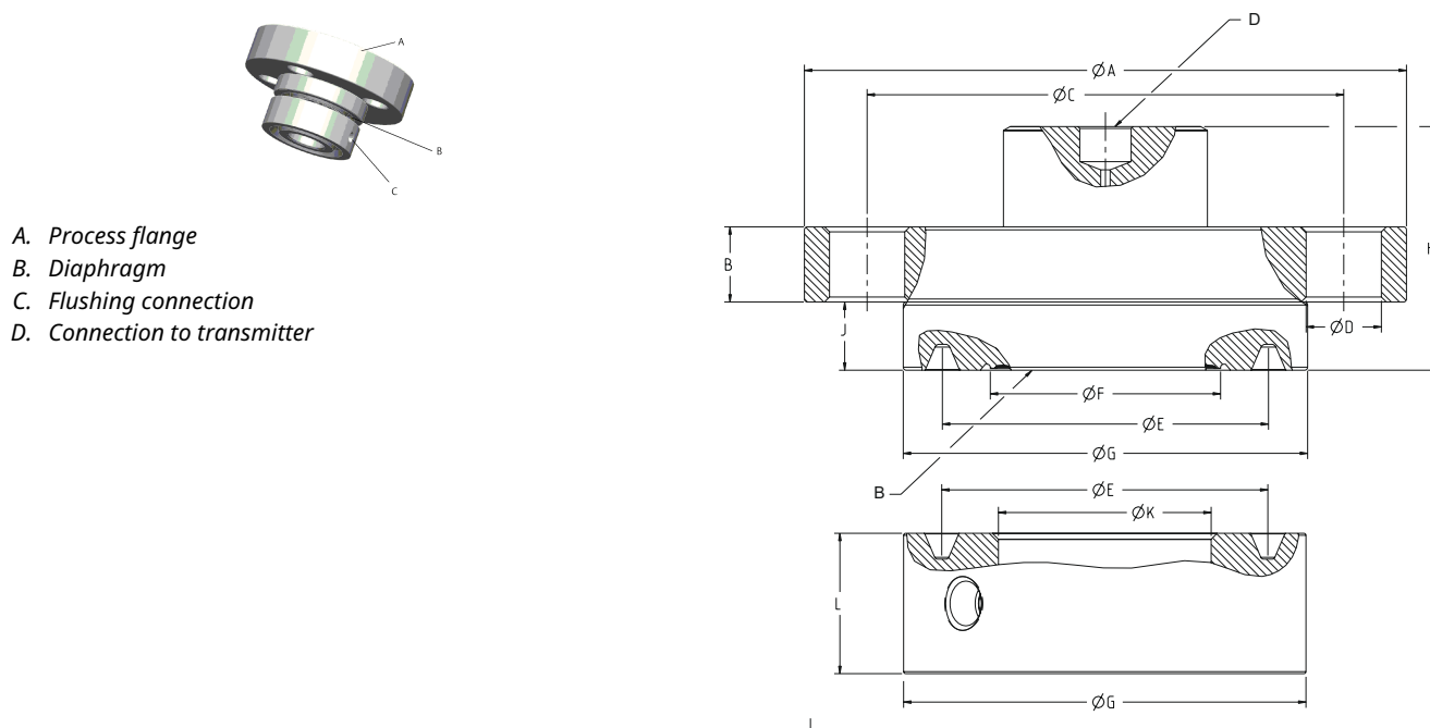
Figure 38: FCW Flush Flanged Seal – RTJ Gasket Surface Two-Piece Design (shown with flushing ring)
