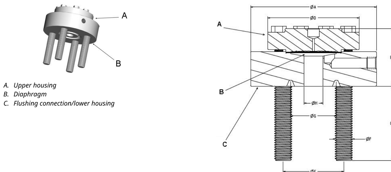
Figure 39: RCW Flanged Remote Seal RTJ and Flushing Connection Ring
