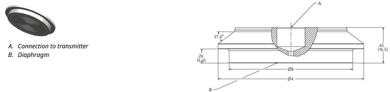
Figure 50: SHP Cherry-Burrell “T” Line Seal
