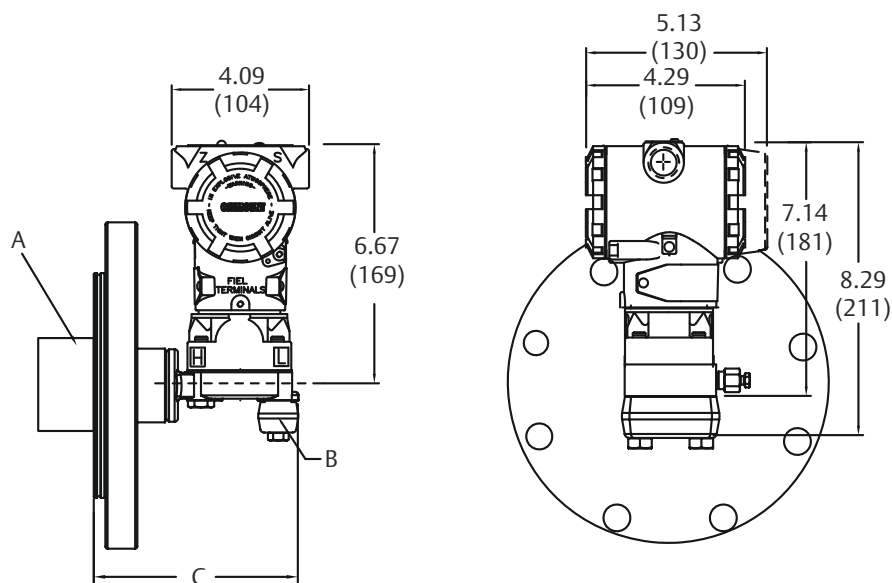
Figure 26: Rosemount 3051L Level Transmitter with FF or EF Seal
