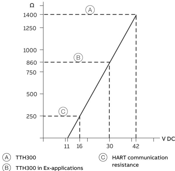
Figure 2: Maximum load depending on Supply voltage
