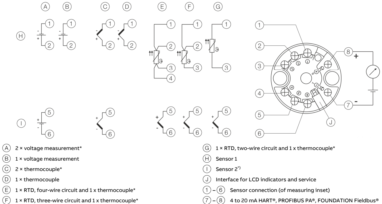
Figure 4: Terminal assignment for thermocouples / voltages and resistance thermometers (RTD) / thermocouple combinations
