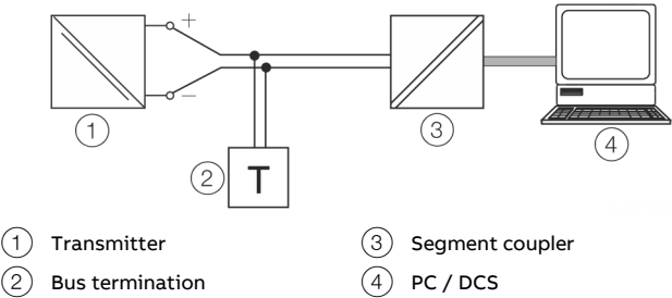
Figure 6: Example of PROFIBUS PA® interface connection
