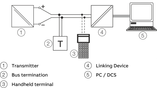
Figure 7: Example of FOUNDATION Fieldbus® interface connection
