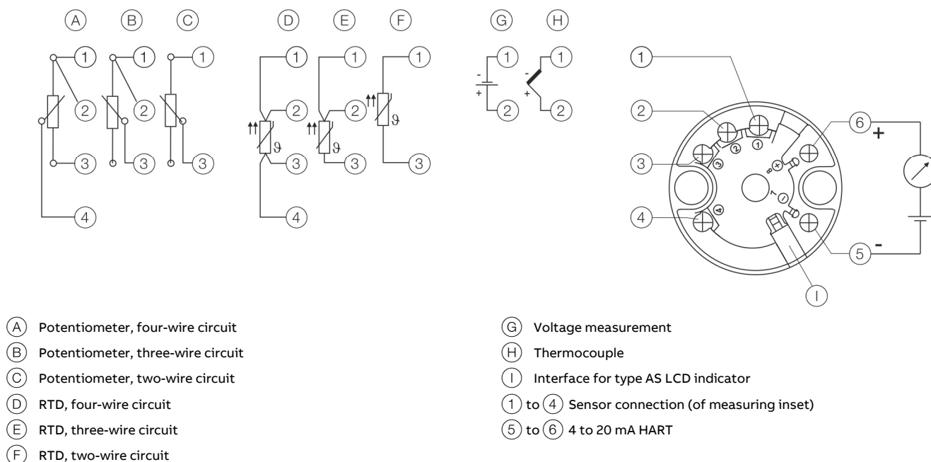
Figure 3: TTH200 connections
