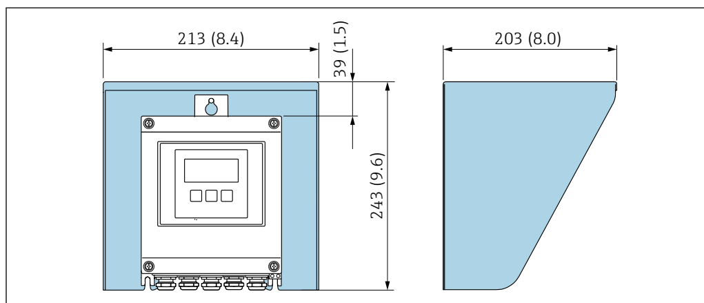
31 Weather protection cover; engineering unit mm (in)
