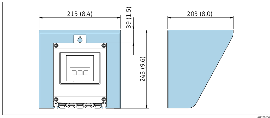
18 Weather protection cover; engineering unit mm (in)
