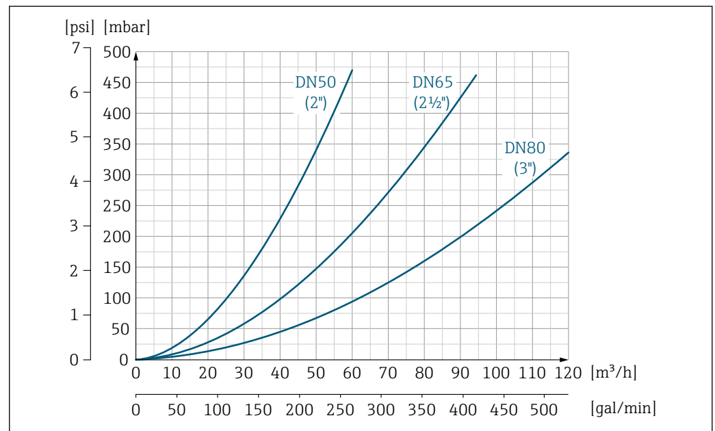
29 Pressure loss DN 50 to 80 (2 to 3") for order code for "Design", option C "Fixed flange, constricted measuring tube", 0 x DN inlet/outlet runs"
