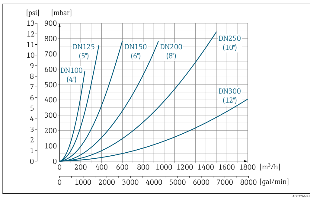
30 Pressure loss DN 100 to 300 (4 to 12") for order code for "Design", option C "Fixed flange, constricted measuring tube", 0 x DN inlet/outlet runs"
