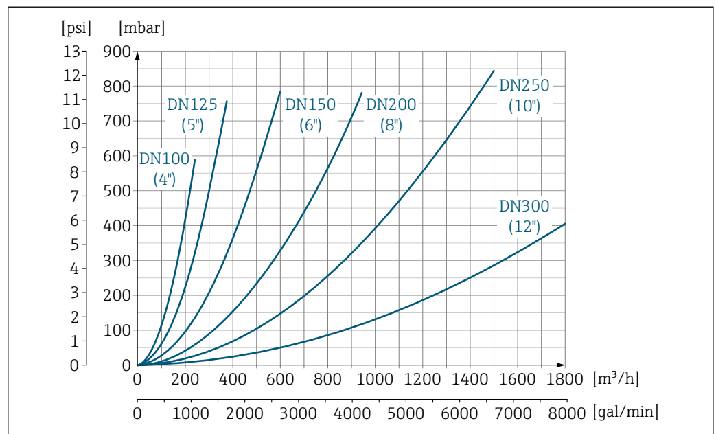
25 Pressure loss DN 100 to 300 (4 to 12") for order code for "Design", option C "Fixed flange, constricted measuring tube", 0 x DN inlet/outlet runs"
