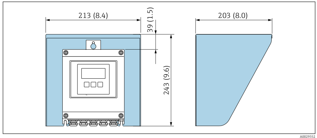
14 Weather protection cover; engineering unit mm (in)
