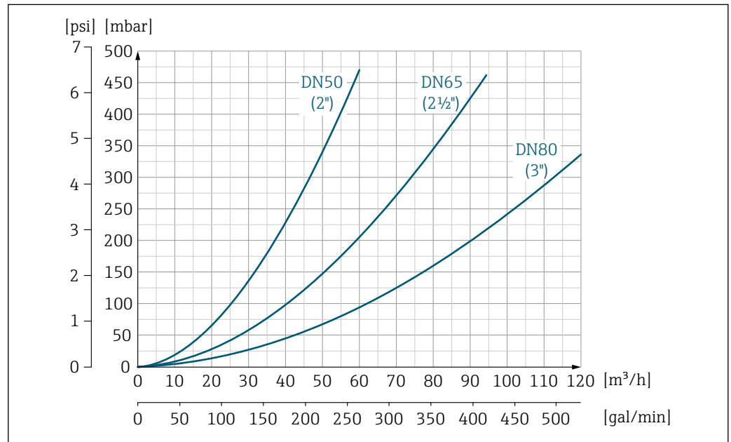
24 Pressure loss DN 50 to 80 (2 to 3") for order code for "Design", option C "Fixed flange, constricted measuring tube", 0 x DN inlet/outlet runs"
