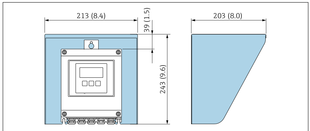
26 Weather protection cover; engineering unit mm (in)
