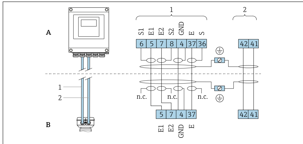
6 Remote version terminal assignment
