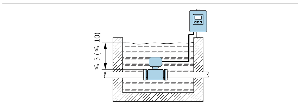
15 Installation for permanent immersion in water
