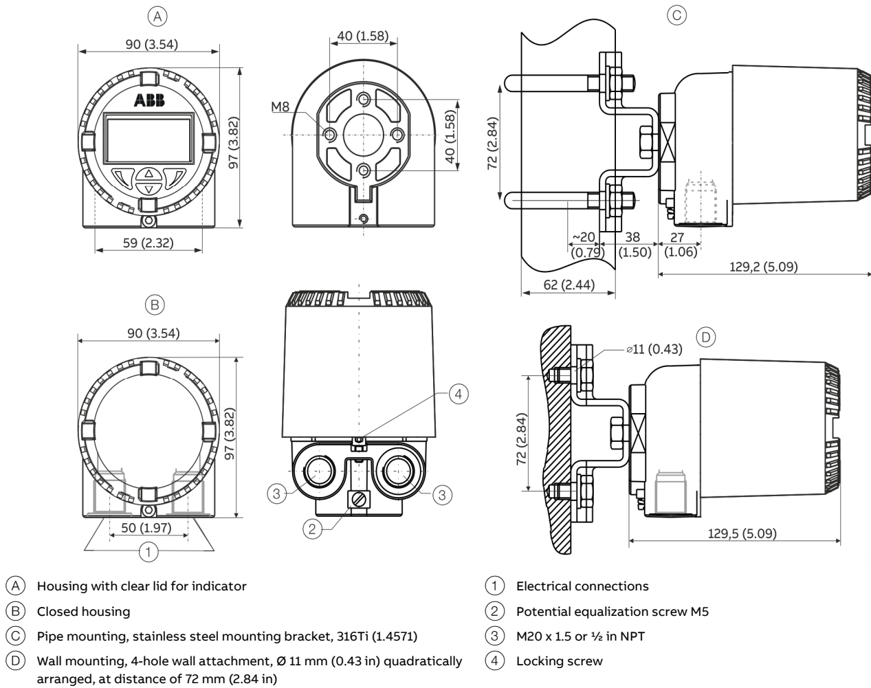
Figure 8: Dimensions in mm (in)
