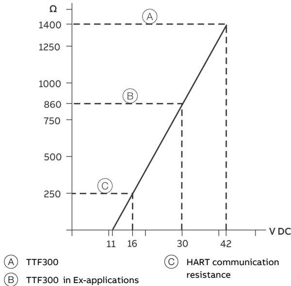
Figure 2: Maximum load depending on Supply voltage
