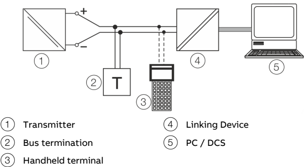
Figure 7: Example of FOUNDATION Fieldbus® interface connection
