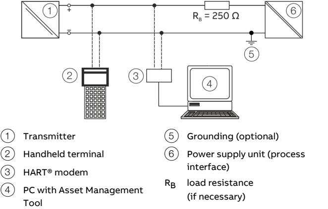
Figure 5: Example of HART® interface connection
