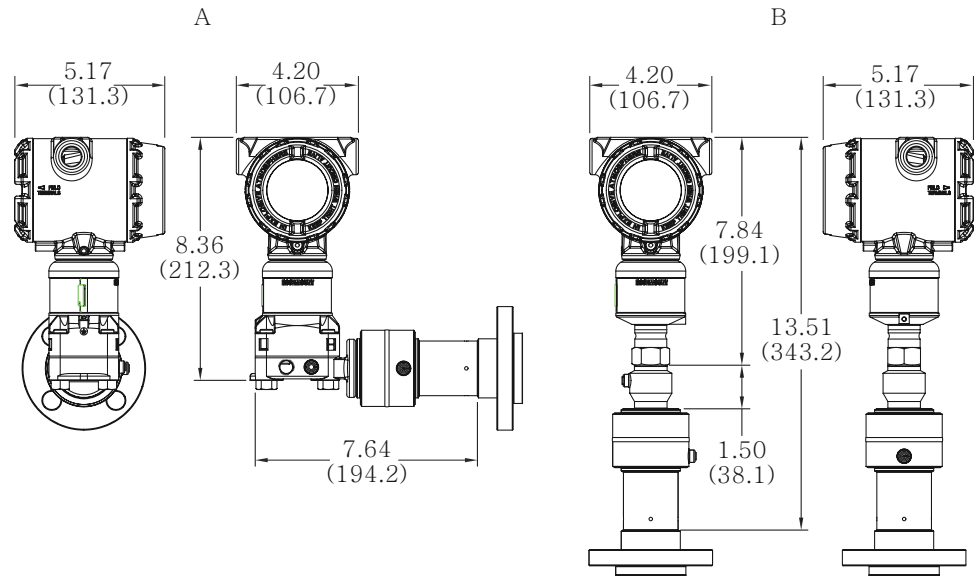
Figure 31: Rosemount 3051S Scalable Level Transmitter with Thermal Range Expander
