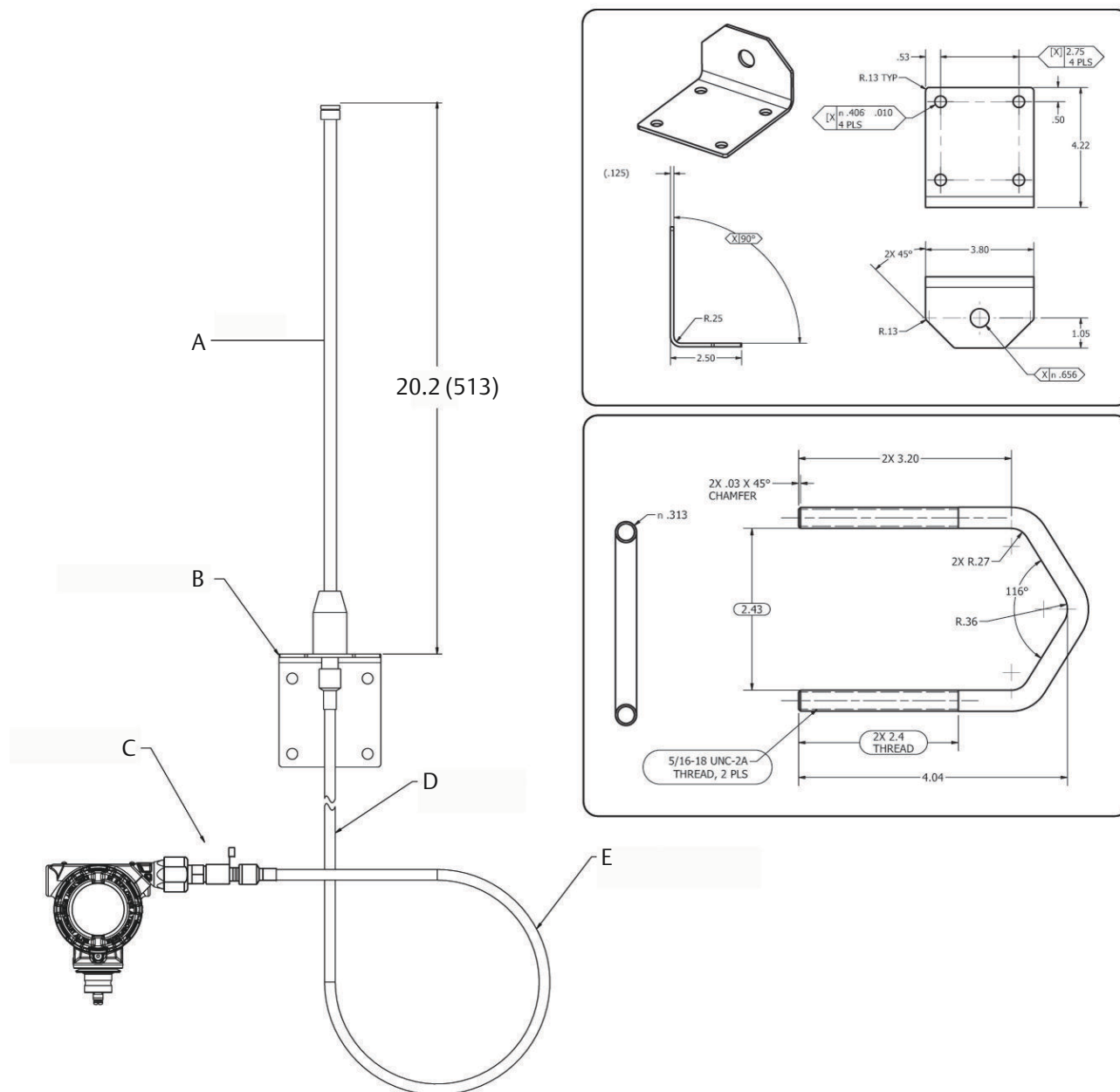
Figure 16: High Gain, Remote Mount Antenna (WN Option)
