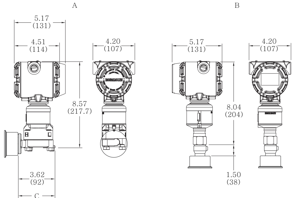
Figure 30: Rosemount 3051S Scalable Level Transmitter with SC Seal
