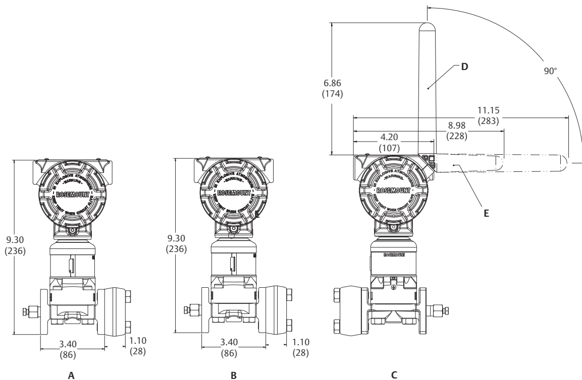
Figure 12: Transmitter with Coplanar Sensor Module and Traditional Flange (Front View)
