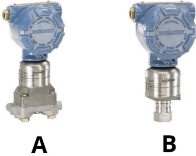
Figure 1: 3051SAM
