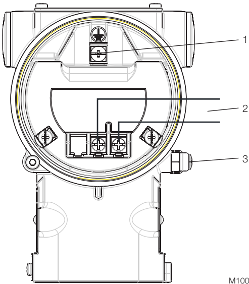
Fig. 7: Standard terminal strip 1 Internal ground termination point | 2 Fieldbus line (polarity independent) | 3 External ground termination point
