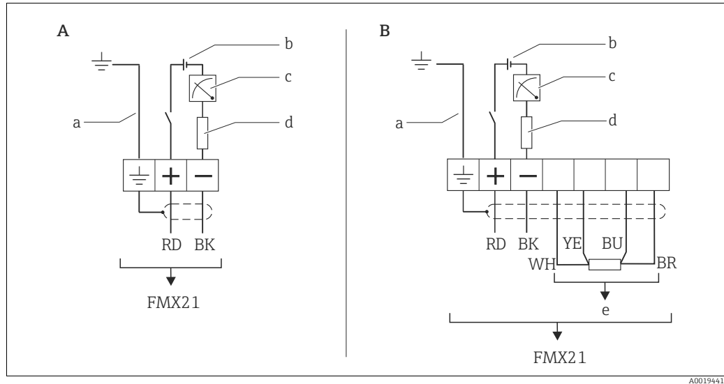
A Waterpilot FMX21
