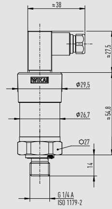
Angular connector DIN 175301-803 A with zero point adjustment ring
