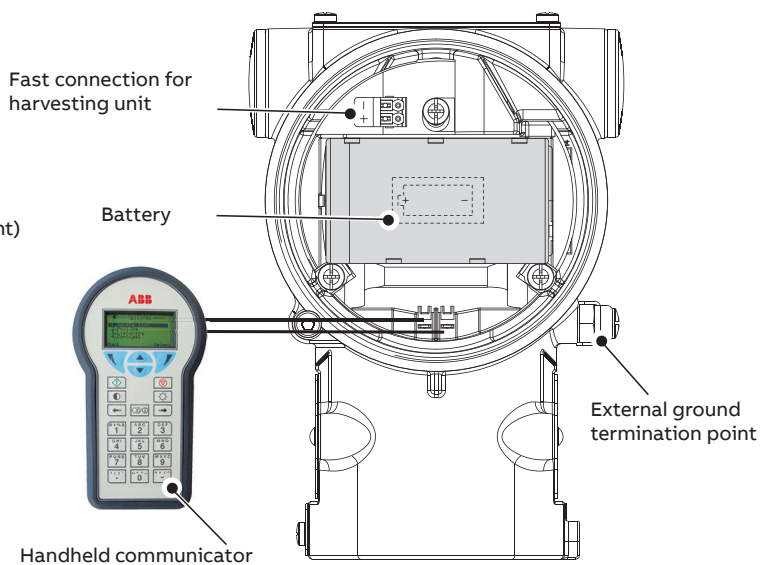
Figure 13 WirelessHART version
