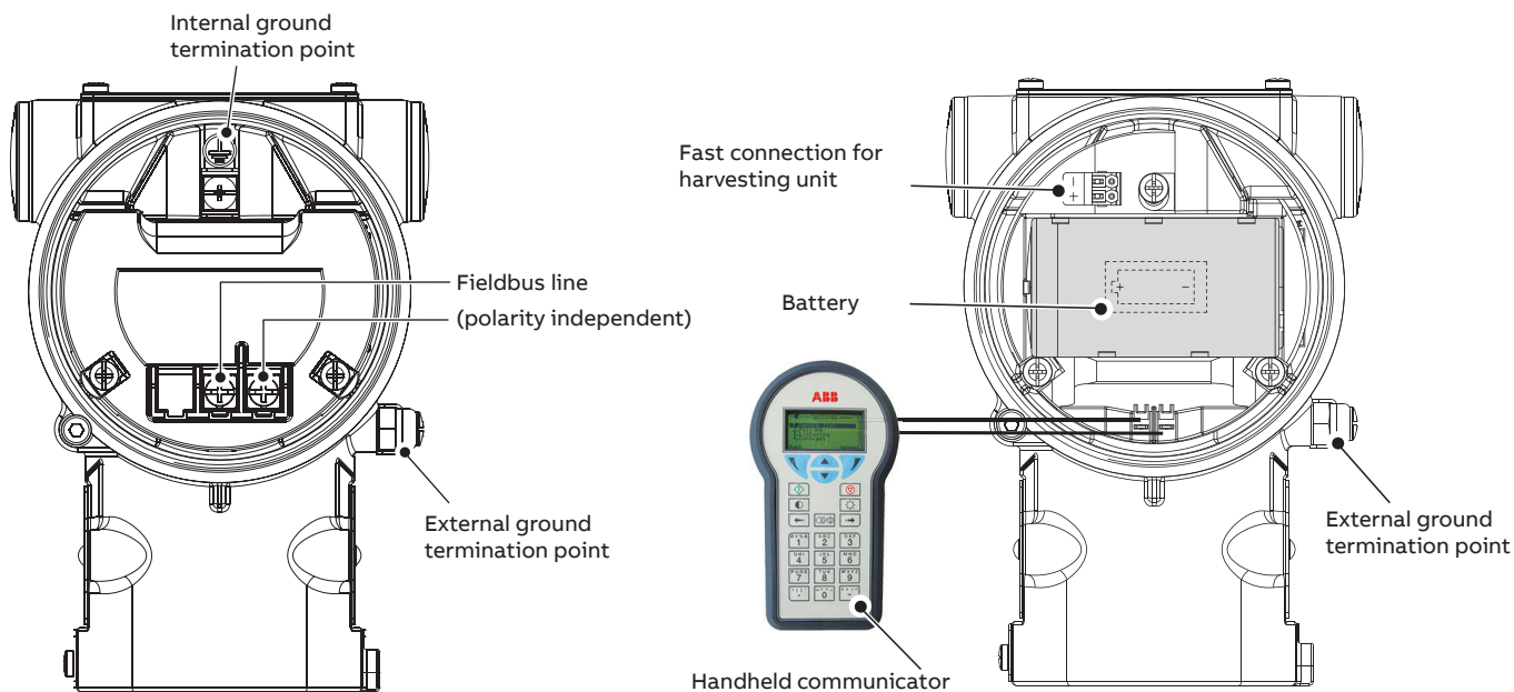
Figure 11 FIELDBUS Versions
