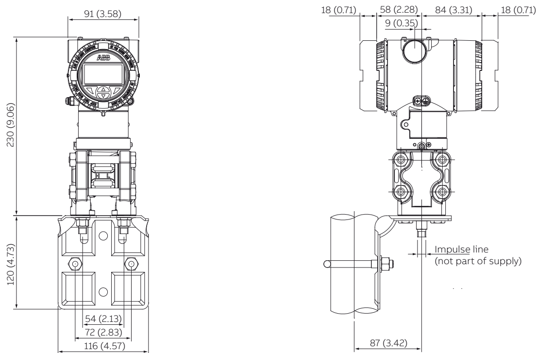
Figure 2 Standard static transmitter with barrel housing - vertical flanges
